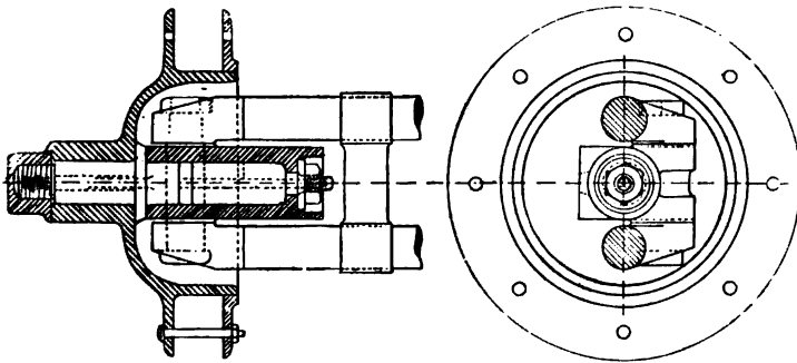
FIG 40.—The Cluibe and Southey Pivoted Steering Hub used on the Carriages of the Electric Motive Power Co., of England. As may be seen, the pivot is to one side of the axle, thus giving the wheel a true caster movement in turning.
